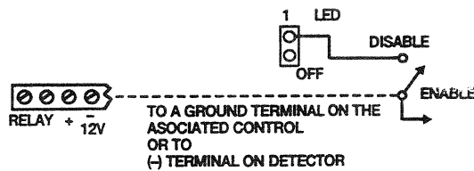
Figure 2. Remote Control of LED
