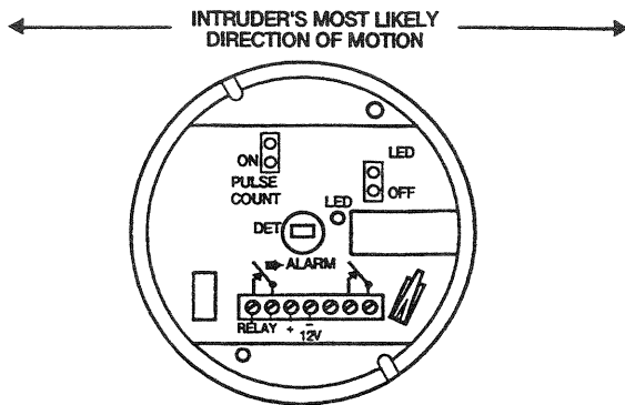
Figure 1. Optimum Mounting Orientation
